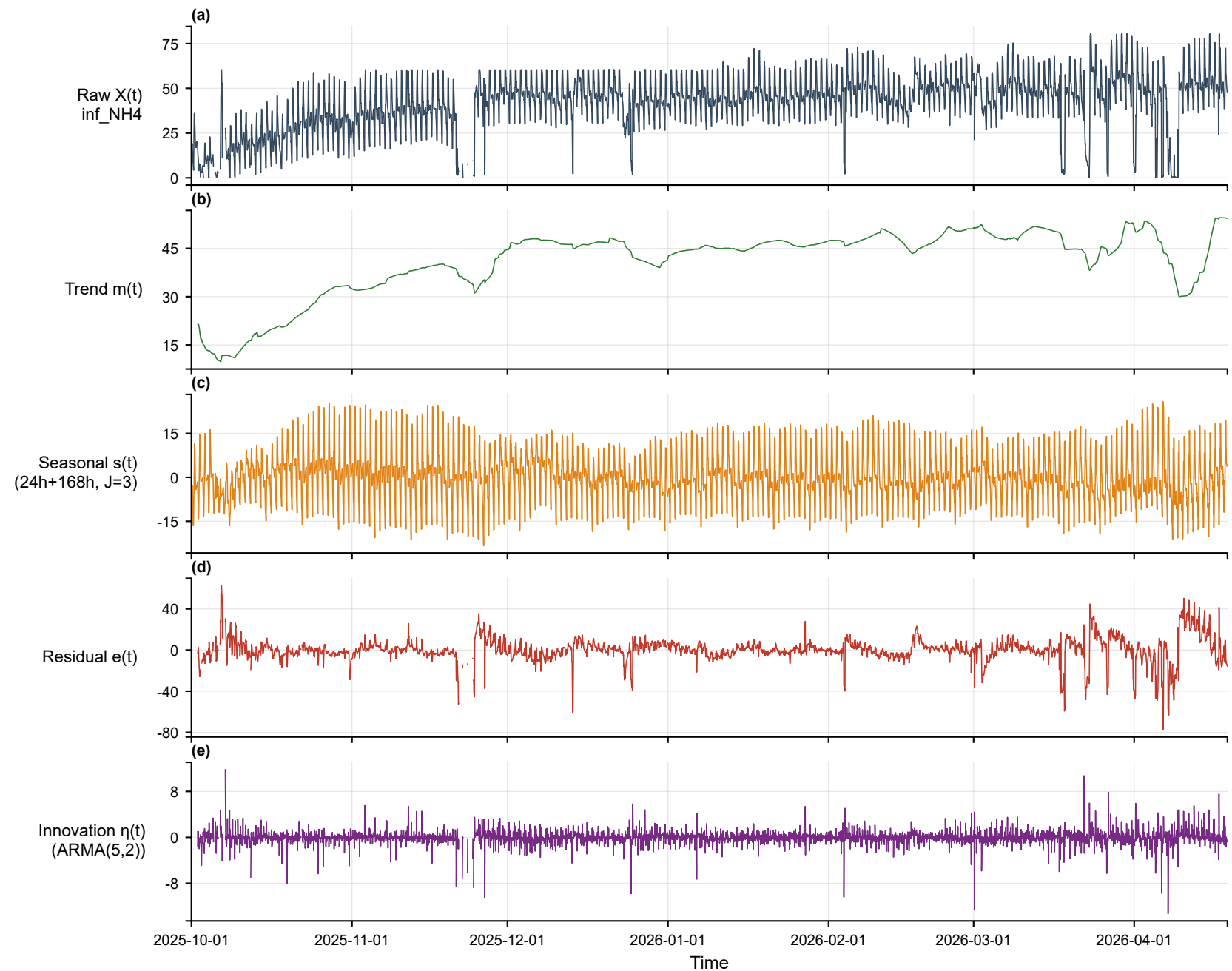
Multi-scale decomposition — inf_NH4 (influent, hour) [2025-10-01~2026-04-19]
